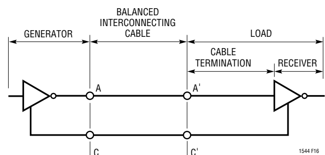
Figure 16. Typical V.28 Interface
